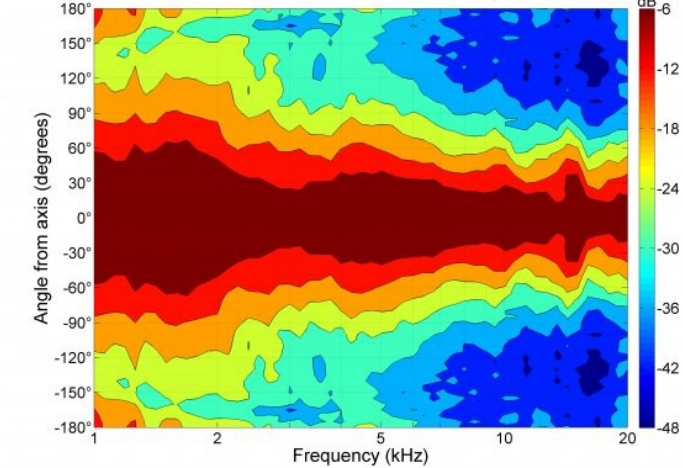
15HCX76 HF vertical directivity map
