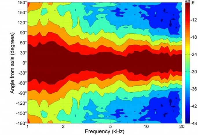
15HCX76 HF horizontal directivity map
